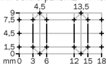
AHx Control panel x2 - RP 18x9
