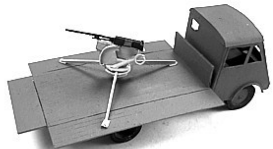
Dedicated "Flak" open cargo bed (Breda 20/65 is detailed in Booklet n°9).
